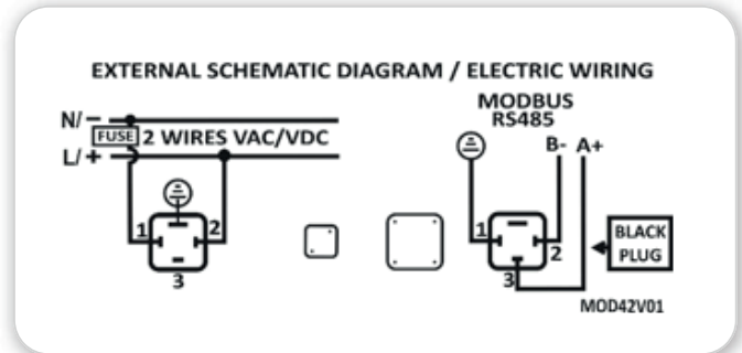
Wiring diagram J4C 140 - 300 + Modbus
